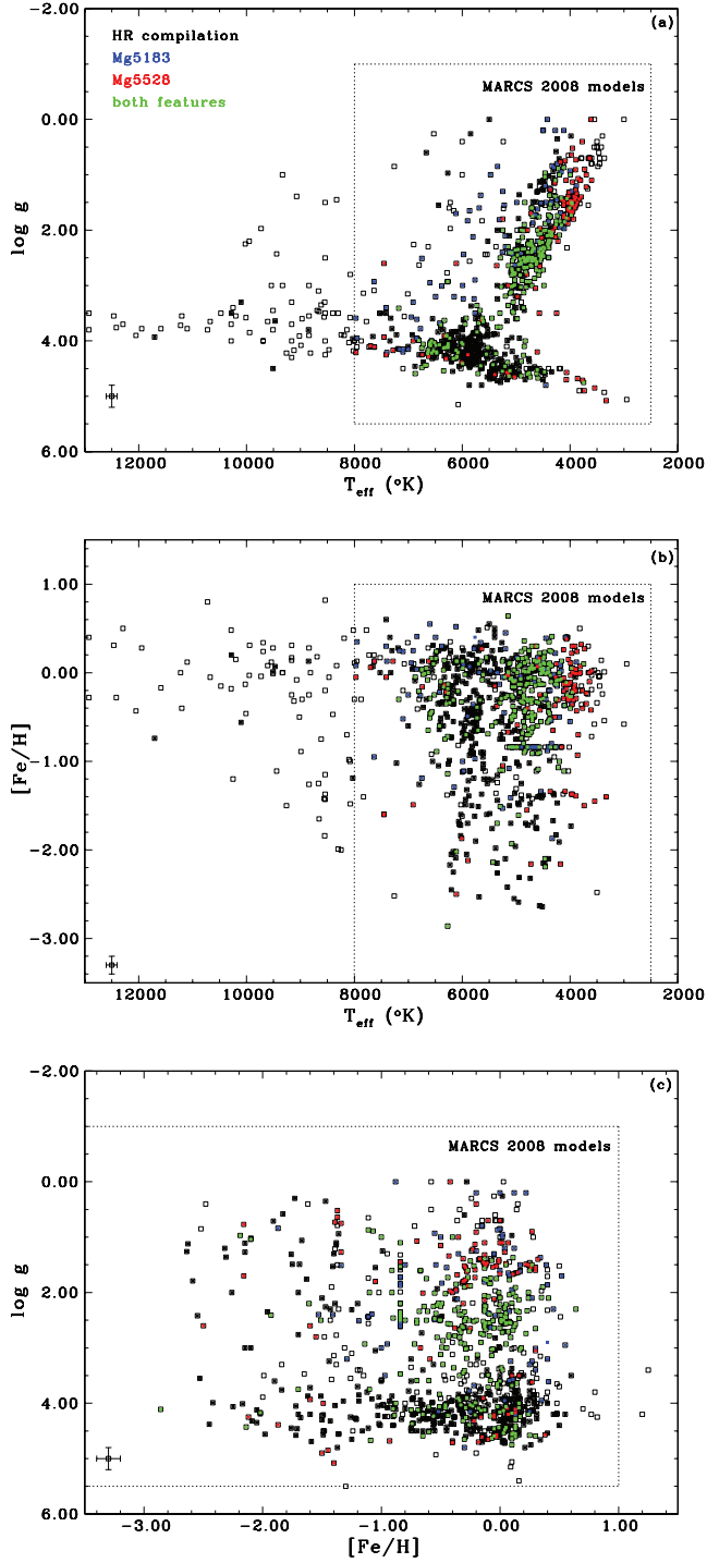
Figure 7. Coverage of the MILES stars with [Mg/Fe] in the photospheric parameter space: (a) modified H-R diagram \log g versus T_{\text{eff}} (top panel), (b) [Fe/H] versus T_{\text{eff}} plane (middle panel) and (c) \log g versus [Fe/H] projection (bottom panel). The MILES stars with abundance ratios from HR studies are shown as black filled symbols, and the stars with MR measurements from this work as colour filled symbols (blue designating determinations based on the Mg5183 feature only, red on Mg5528 only and green on both Mg features combined). The library stars without [Mg/Fe] are drawn as open symbols. The MARCS 2008 grid extension is also represented in each panel.
