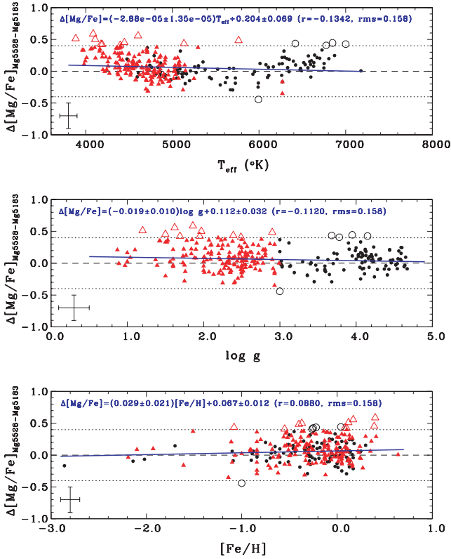
Figure 6. [\text{Mg}/\text{Fe}] differences between the calibrated measurements obtained with the two Mg features ( \Delta[\text{Mg}/\text{Fe}]_{\text{Mg528-Mg5183}} = [\text{Mg}/\text{Fe}]_{\text{Mg528}}^{\text{calib}} - [\text{Mg}/\text{Fe}]_{\text{Mg5183}}^{\text{calib}} ) as a function of T_{\text{eff}} , \log g and [\text{Fe}/\text{H}] for dwarfs (black filled circles) and giants (red filled triangles). LSQ linear fittings between the differences and each photospheric parameter are also shown (solid blue lines) considering the data shown as filled symbols. Two parallel dotted black lines are drawn to representing the 4\sigma [\text{Mg}/\text{Fe}]_{\text{calib}} as a maximum acceptable deviation for \Delta[\text{Mg}/\text{Fe}]_{\text{Mg528-Mg5183}} (details in the end of Section 3.5). The black open circles represent the dwarfs and red open triangles the giants for which average abundance ratios were not computed based on the 4\sigma criterion. These stars are not considered in the LSQ fittings.
