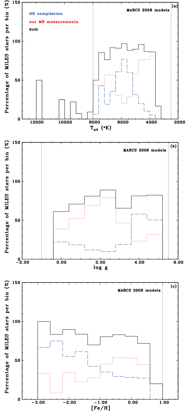
Figure 8. Distribution of the MILES stars with [Mg/Fe] over the photospheric parameter space: (a) effective temperature scale (top panel), (b) surface gravity scale (middle panel) and (c) metallicity scale (bottom panel). The percentage number per bin of the MILES stars with abundance ratios from HR studies is shown by blue dashed line, and the percentage number of stars with our MR measurements by the red dotted line. The sum of both is represented by the black solid line. The adopted bins are equal to four times the parameter uncertainties. The coverage of the MARCS 2008 grid of model atmospheres is also drawn in each panel.
